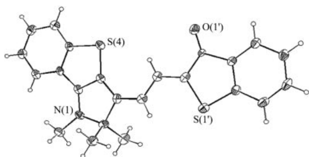
Figure 1. Molecular structure of the cyanine dye 6 . Ellipsoids are drawn at the 20% probability level.
