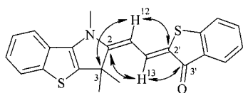
Figure 2. HMBC interactions in cyanine 5 .
