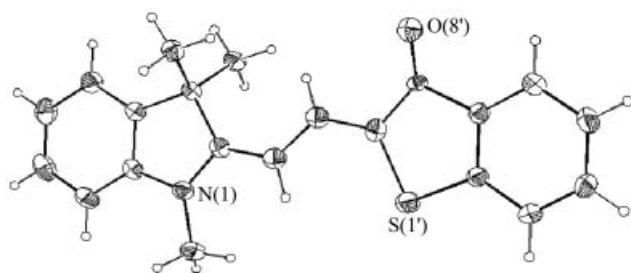
Figure 5. Molecular structure of the cyanine dye 8 . Ellipsoids are drawn at the 20% probability level.
