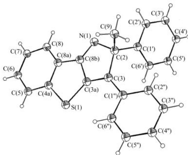
Figure 6. Molecular structure and atom labeling of the 2 H -benzothienopyrrole 9b . Ellipsoids are drawn at the 20% probability level.
