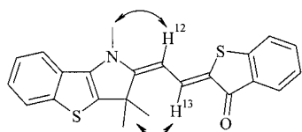
Figure 3. NOESY interactions in cyanine 5 .
